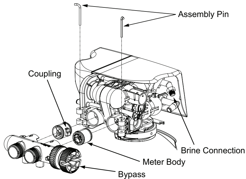
Figure 14. Bypass valve assembly.
