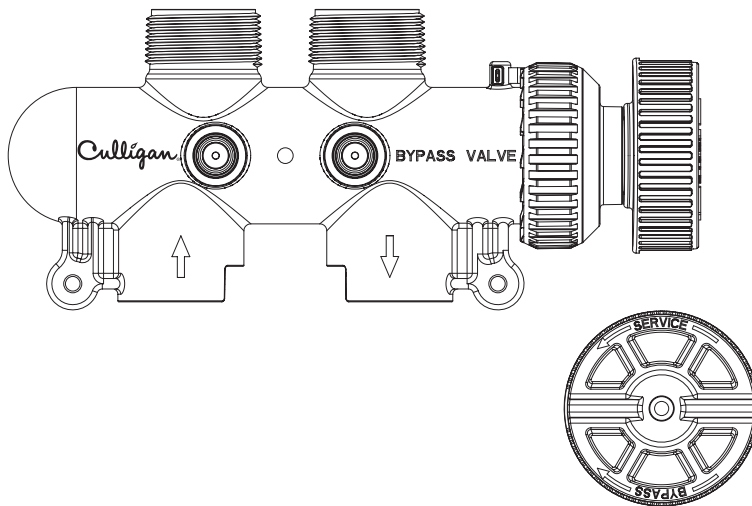
Figure 22. Bypass valve.
