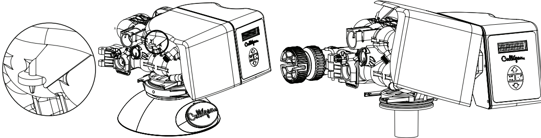
Figure 7. HE softener cover fastener clip.
