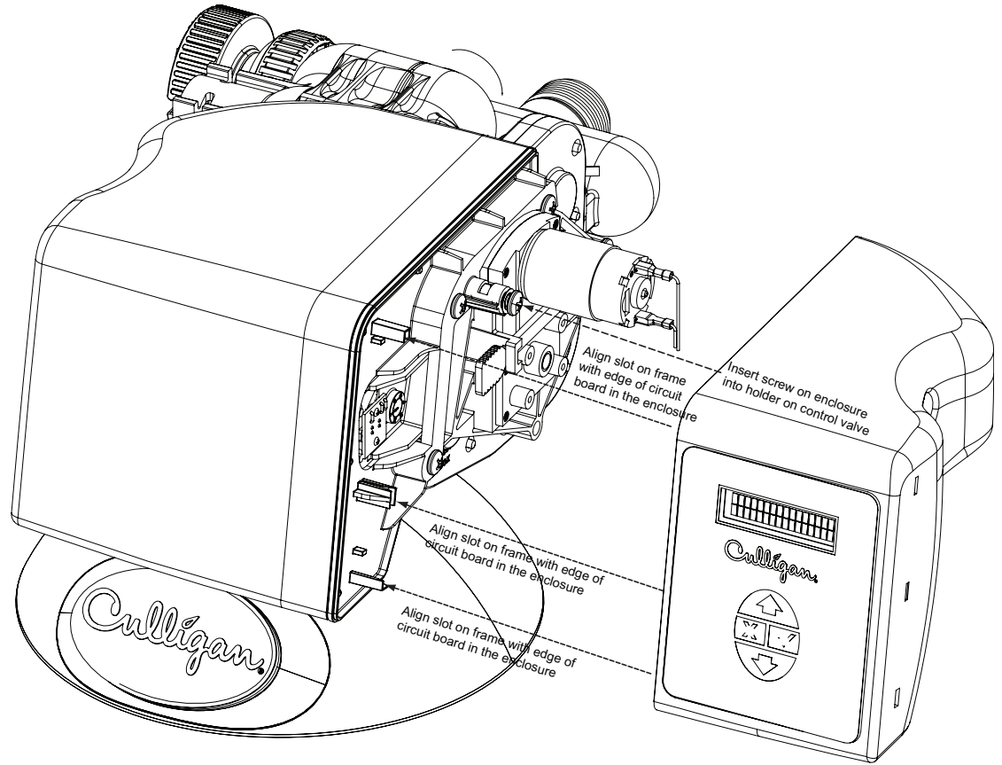
Figure 21. Attaching enclosure cover to control valve.
