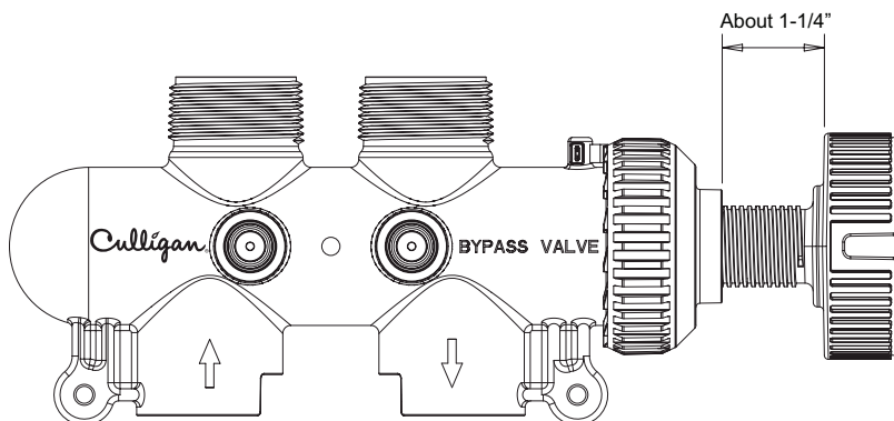
Figure 23. Service valve.
